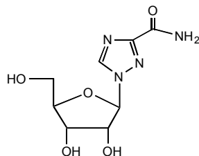
Figure 1: Structural Formula
